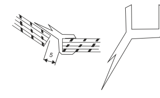
Glass to Glass 135° For 8/10/12mm Size-2200mm Finish-Transparent PCS
