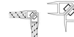
Glass to Glass 90° (Magnetic) For 8/10/12mm (BM) Size-2200mm Finish-Transparent & Black Magnet PCS
