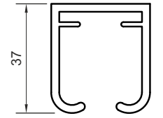
ALU. Profile Size -2400/3000/3600mm Finish -Aluminium
