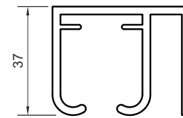
ALU. Profile Size -3600mm Finish -Aluminium
