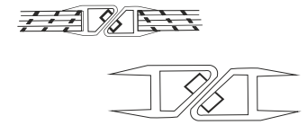
Glass to Glass 180° (Magnetic) For 8/10/12mm (BM) Size-2200mm Finish-Transparent & Black Magnet PCS
