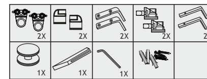
ELITE Shower Sliding glass 1 doors (1 Fix + 1 Sliding Doors)
