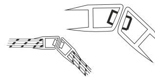
Glass to Glass 135° (Magnetic) For 8/10/12mm (BM) Size-2200mm Finish-Transparent & Black Magnet PCS
