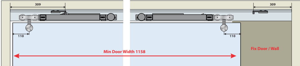
ESLD - 051 DD Two Side Softclose
