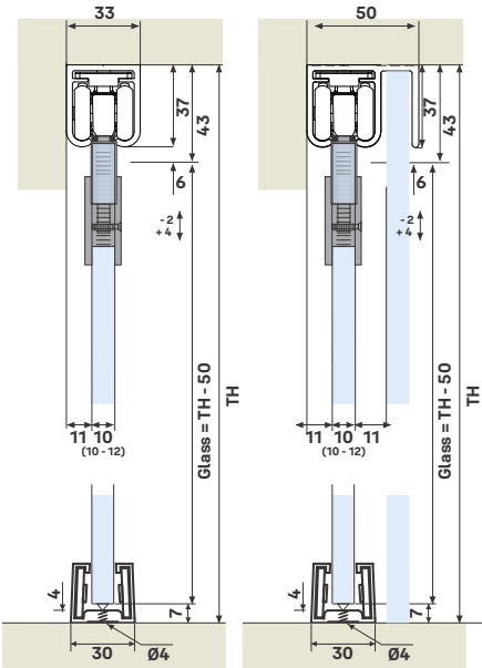
SGSF - 048 A SD One Side Softclose
