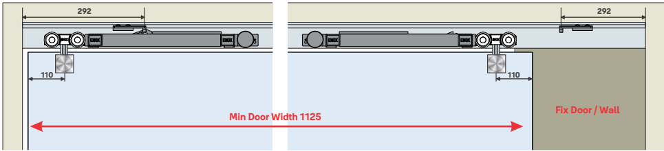
SGSF - 048 A DD Two Side Softclose
