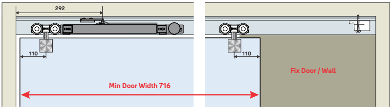
SGSF - 048 A SD One Side Softclose
