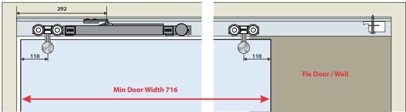
SGSF - 022 A SD One Side Softclose
