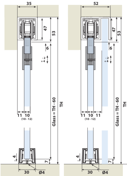
ESLD - 051 SD One Side Softclose
