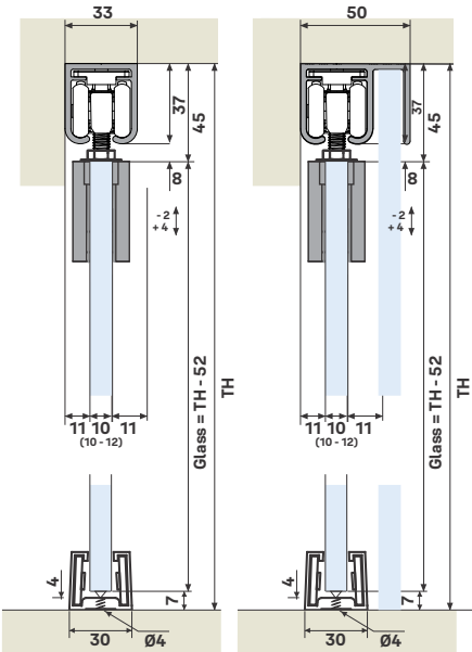
ESLD - 011 A SD One Side Softclose
