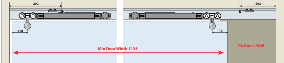
SGSF - 022 A DD Two Side Softclose
