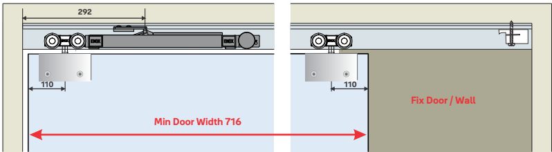
ESLD - 011 A SD One Side Softclose
