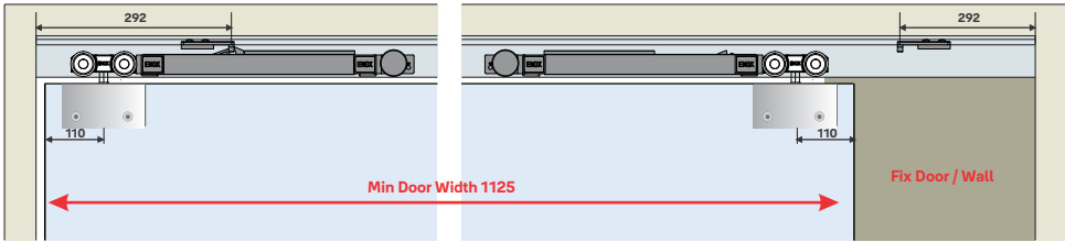
ESLD - 011 A DD Two Side Softclose
