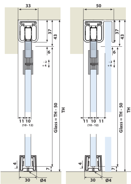
SGSF - 022 A SD One Side Softclose
