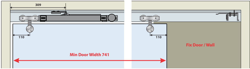
ESLD - 051 SD One Side Softclose
