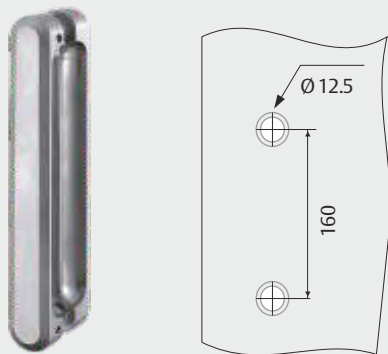
Glass Hole Details
