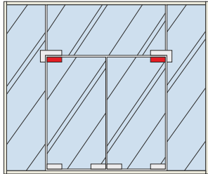
Top patch fitting
