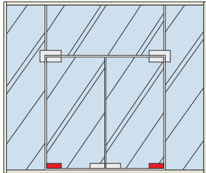
Bottom patch fitting
