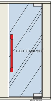
Glass Door Pull Handle With Lock (Square)
