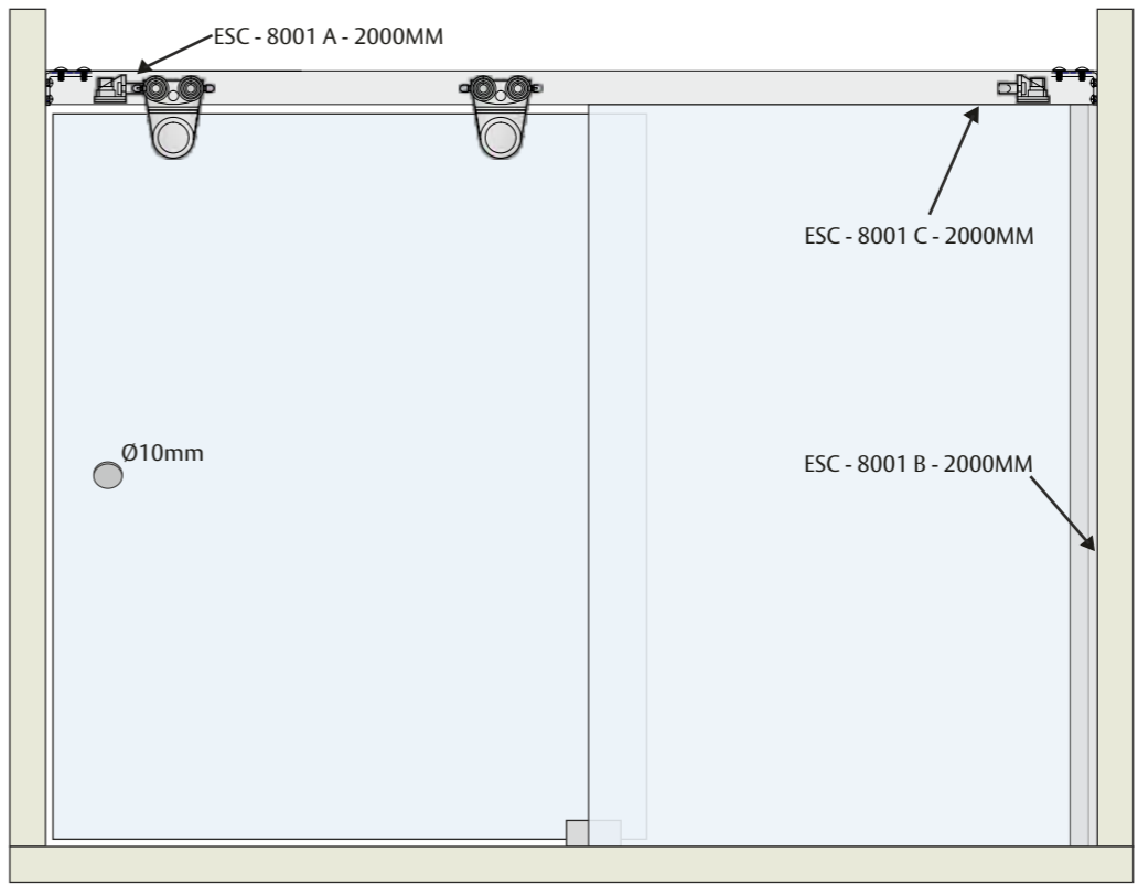
ELITE Shower Sliding Systems
