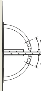
Double Action Spring Return Door From 25° In Each Direction
