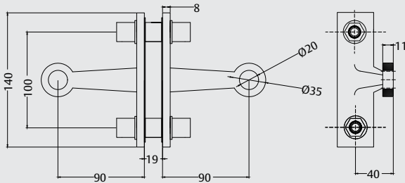
Glass cut-out details
