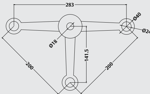
Glass cut-out details
