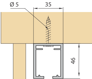
Mounting example
