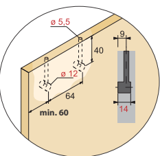
Preparing the door
