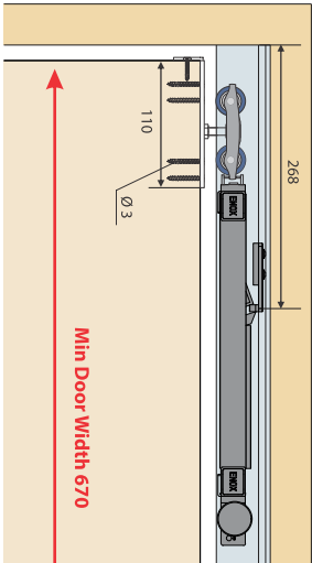
ESLD - 045 SD One Side Softclose
