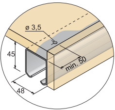
Assembly runner profile
