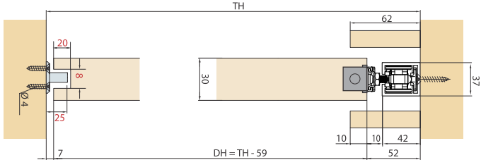
Mounting example
