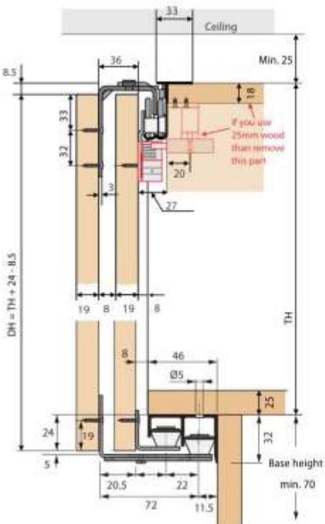
Mounting example
