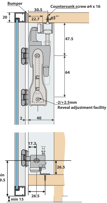
Mounting example
