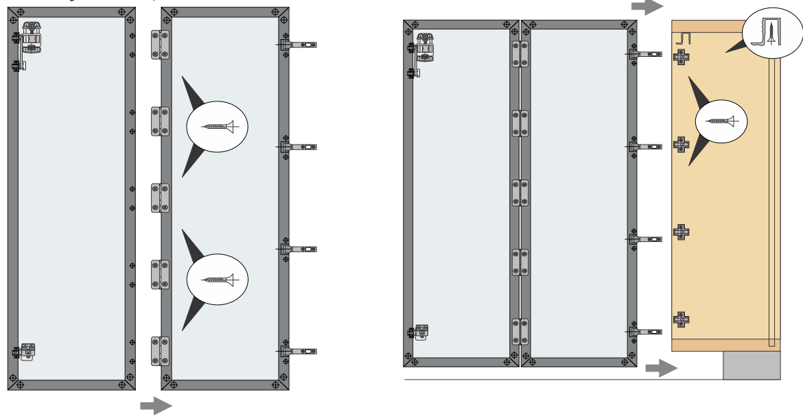
Assembly
