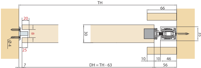
Mounting example
