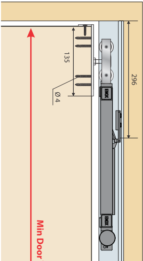
ESLD - 046 DD Two Side Softclose
