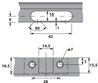
Milling diagram
