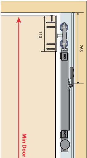
ESLD - 045 DD Two Side Softclose
