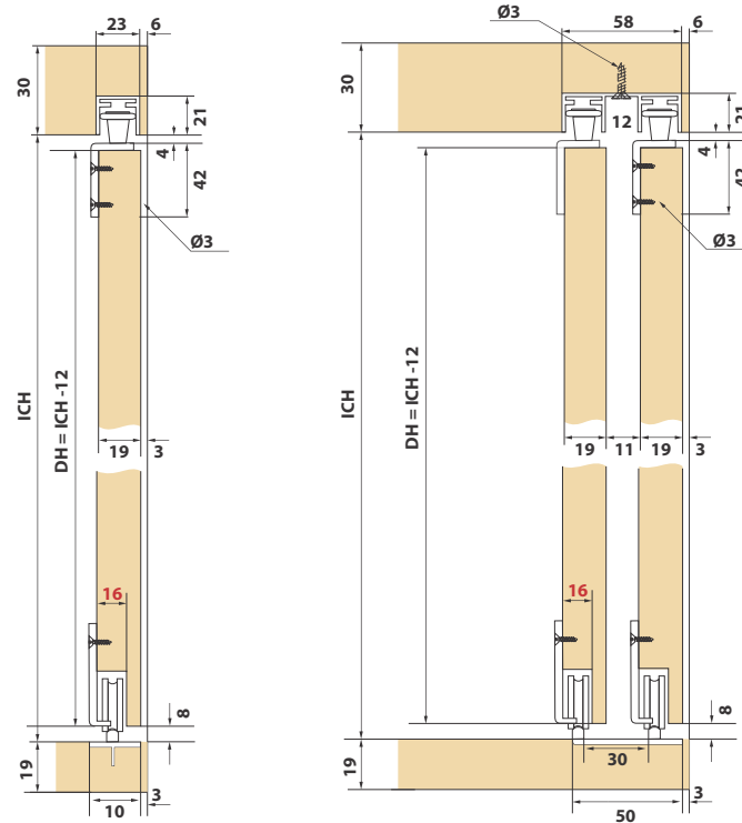
Mounting example
