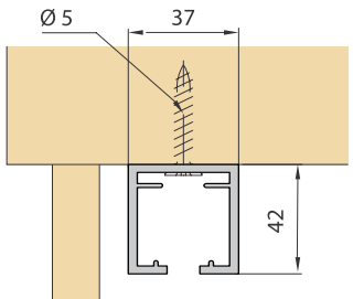
Mounting example
