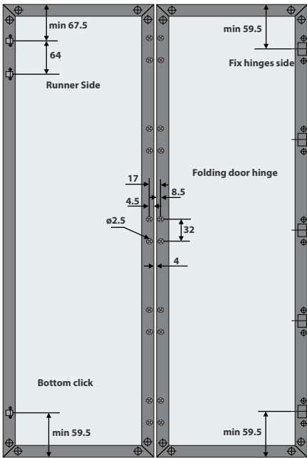
Drilling pattern
