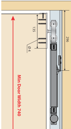
ESLD - 046 SD One Side Softclose
