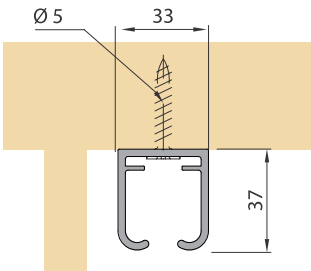
Mounting example
