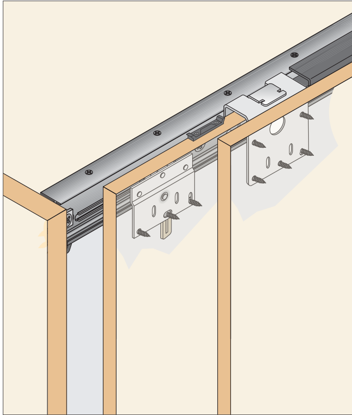
Mounting example
