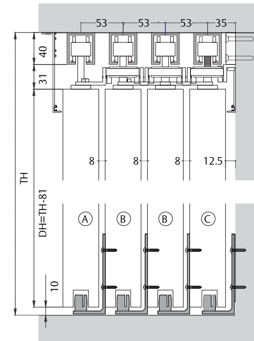
ESLDF 084 / 4 for wooden telescopic 4 sliding panels
