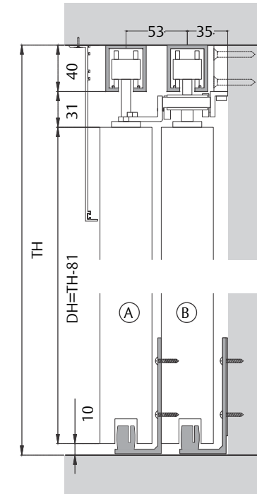
ESLDF 084 / 4 for wooden telescopic 4 sliding panels
