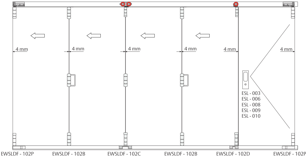
4 sliding panel configuration with 1 door
