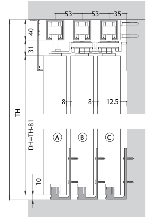
ESLDF 084 / 3 for wooden telescopic 3 sliding panels
