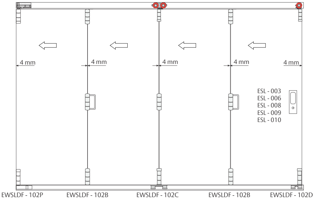
Glass Side Sliding Folding System (with bottom track) Assembly Types 4 sliding panel configuration
