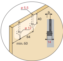
Preparing the door
