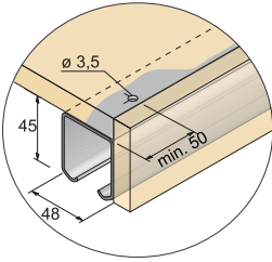
Assembly runner profile
