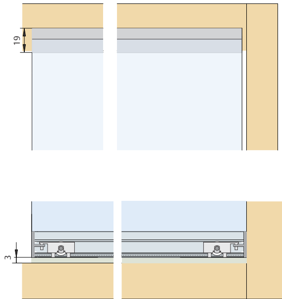
ICW - Internal cabinet width, DH - Door height, ICH - Internal cabinet height
